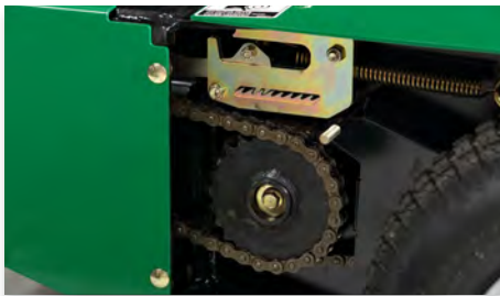
Innovative automatic chain tensoning system reduces the chain maintenance required
