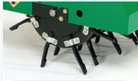
Cast iron aeration wheels have sintered bushings and lubrication fittings for durability and easy maintenance.
