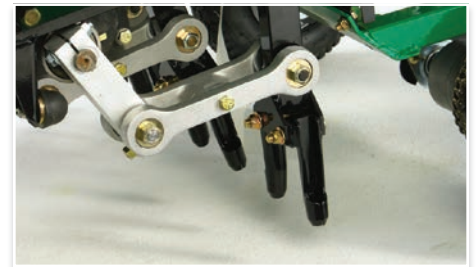
Reciprocating tines provide vertical coring action, punching straight in and out without tearing the turf, offering quality on par with golf courses.
